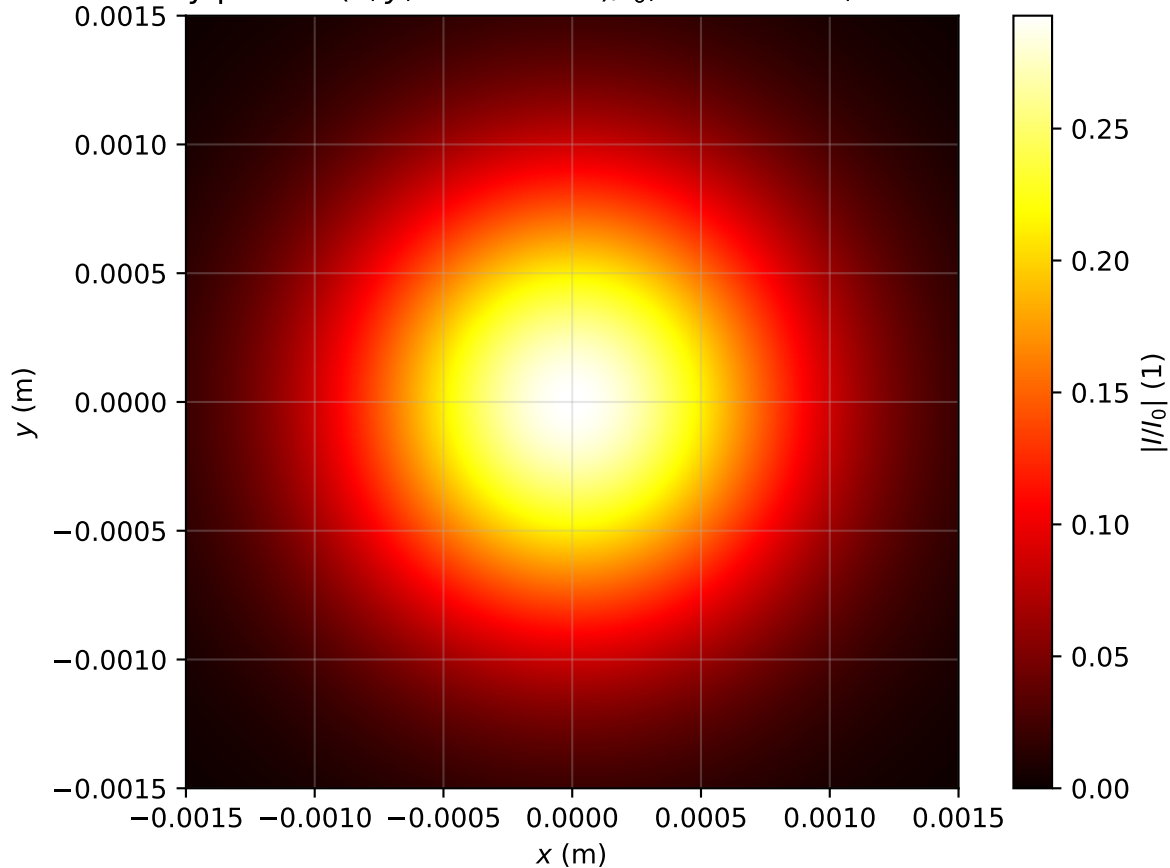
Intensity profile I(x, y, z = 3.901m)/I_0 , P_{in}=0.3P_{cr} , artificial time
